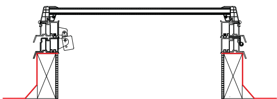
Electric opening to fit to builder's upstand
