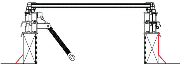
Manual opening to fit to builder's upstand
